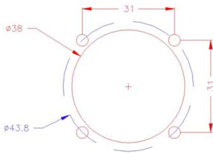
Punching details
