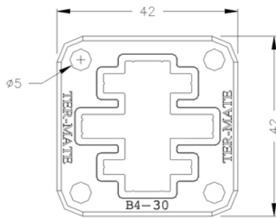
Overall dimensions
